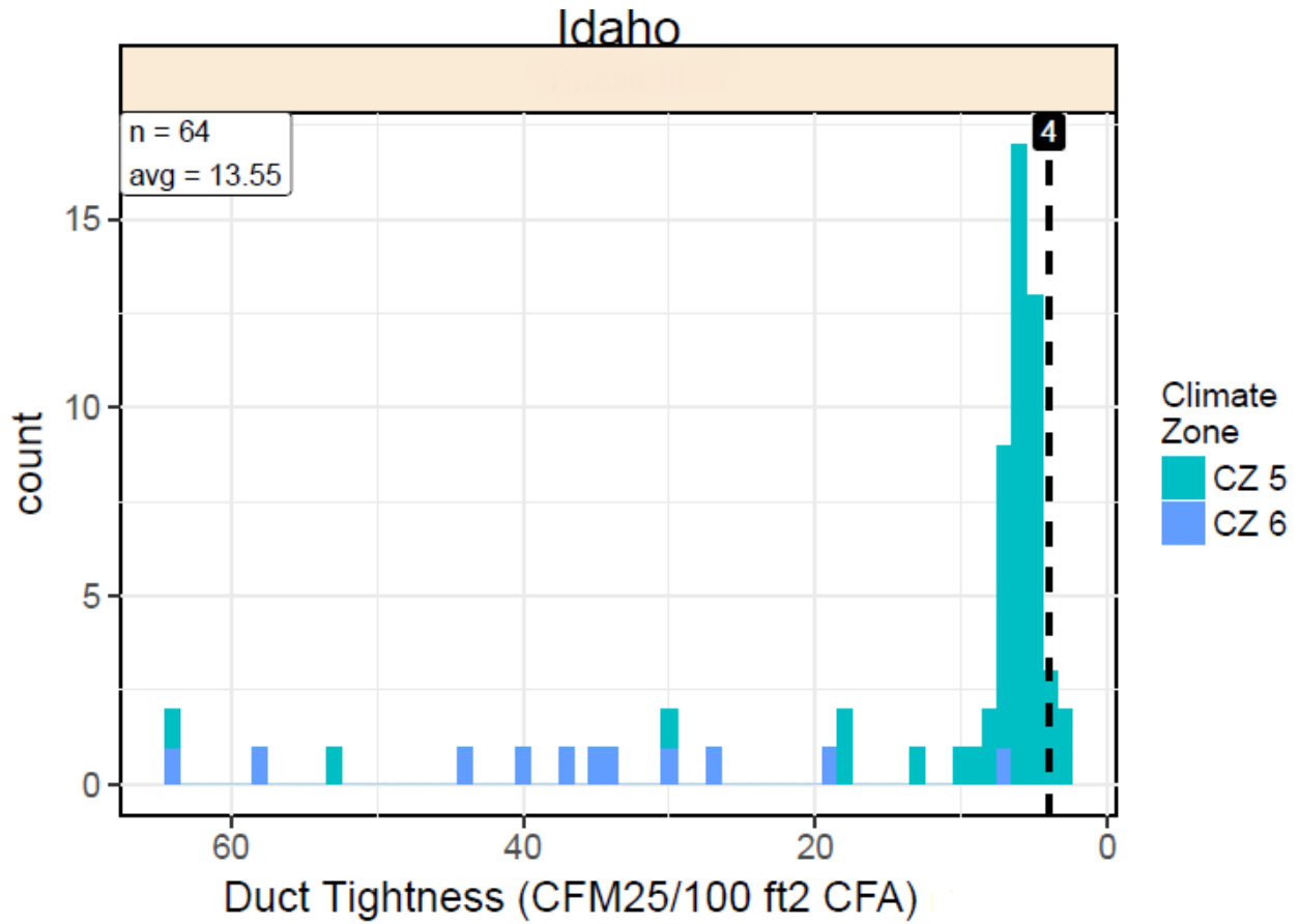
Figure 3.14. Raw Duct Tightness (CFM25/100ft2 CFA)
