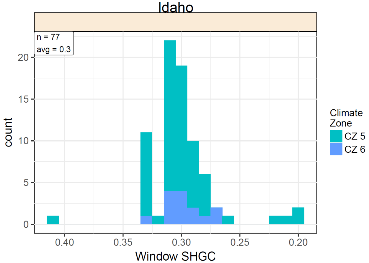
Figure 3.2. Window SHGC
