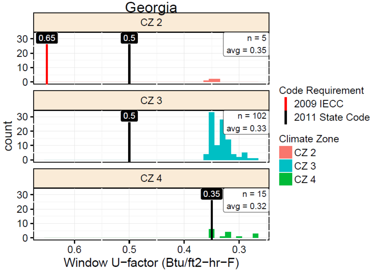
Figure 3.3. Window U-Factor
